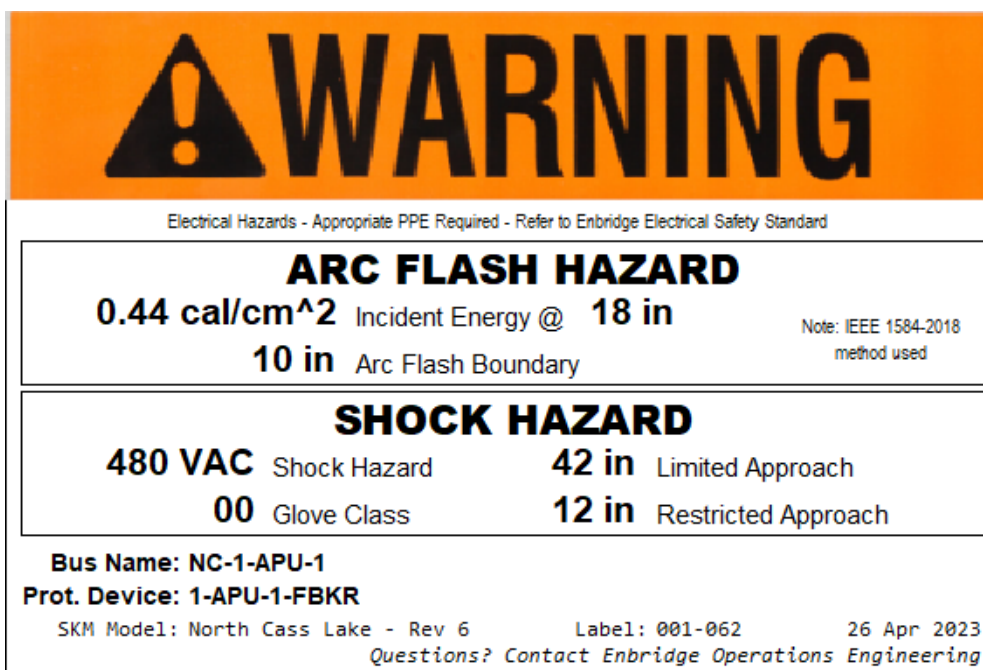
Figure 3 – (LP Only) Sample Detailed Arc Flash and Shock Warning Label
